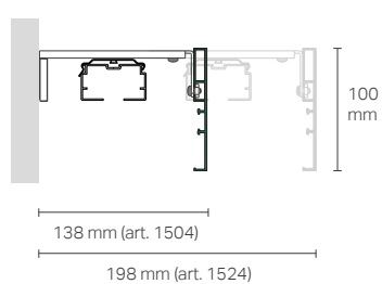
Attacco a parete Wall mount
