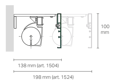
Attacco a parete Wall mount
